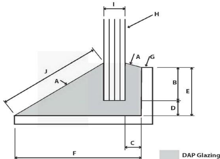
Illustration of Key Terminology Used in Face Glazing
